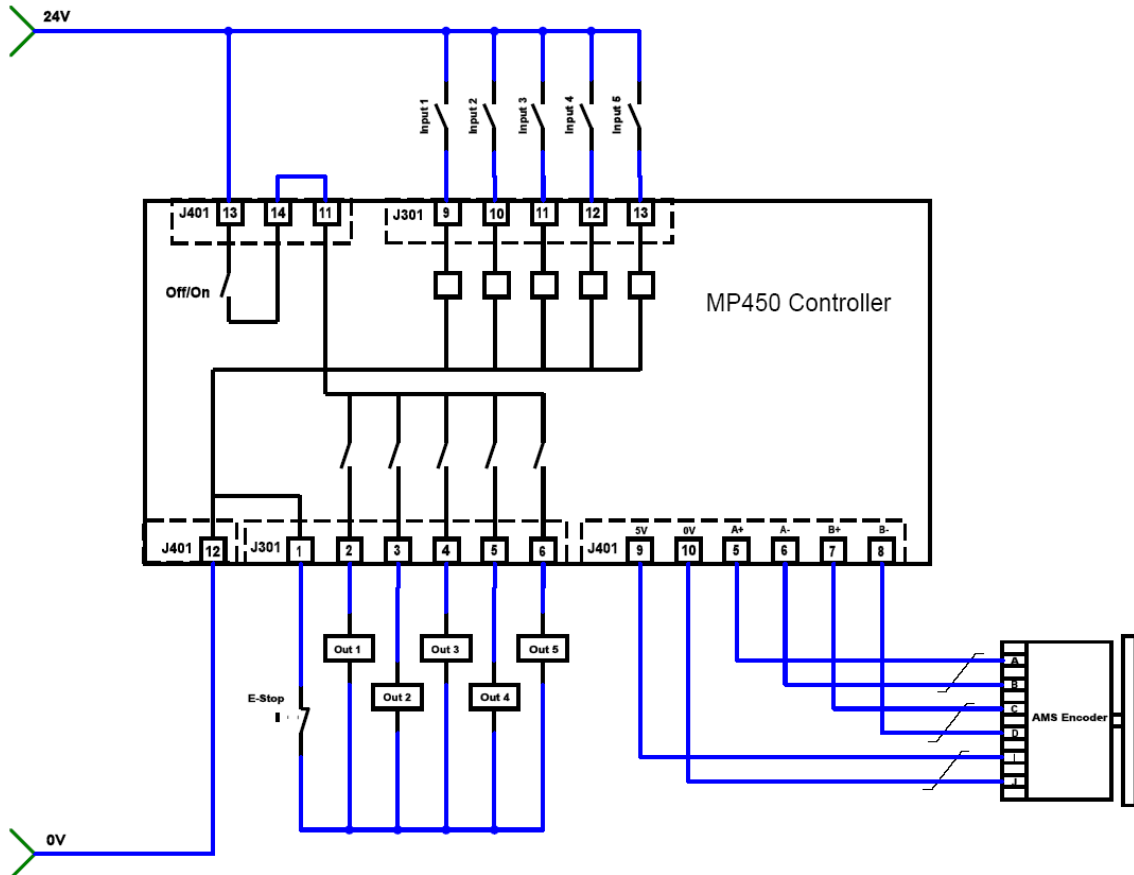
Figure 4: MP465 Sample Interface Drawing
