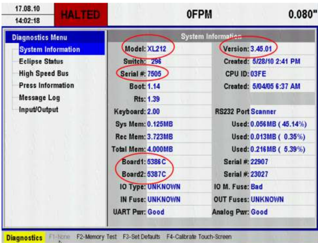
XL200 System Information Menu
