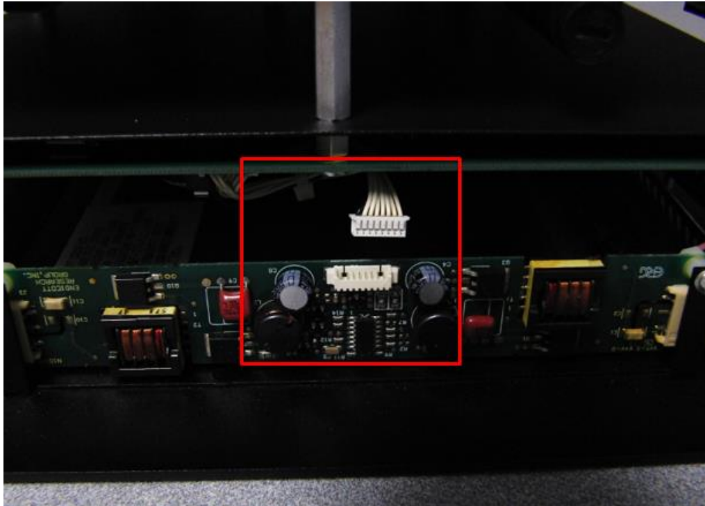
Figure 7 - White connector removed
