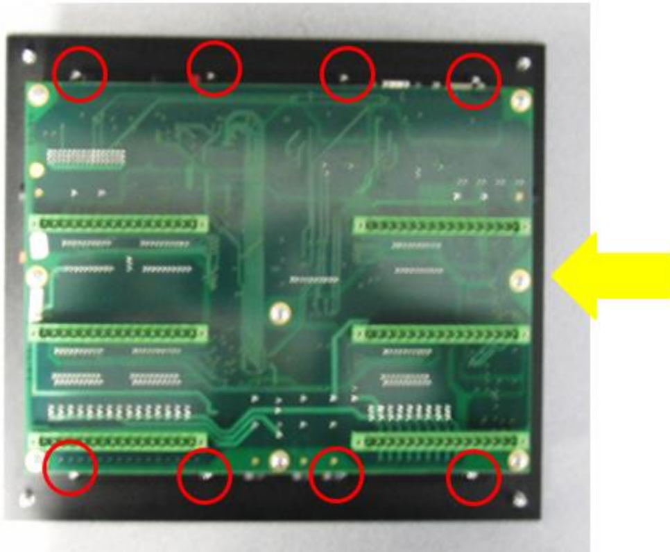
Figure 6 - XL200 with back cover removed
